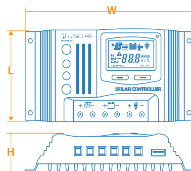
▶ Dimension reference drawing
